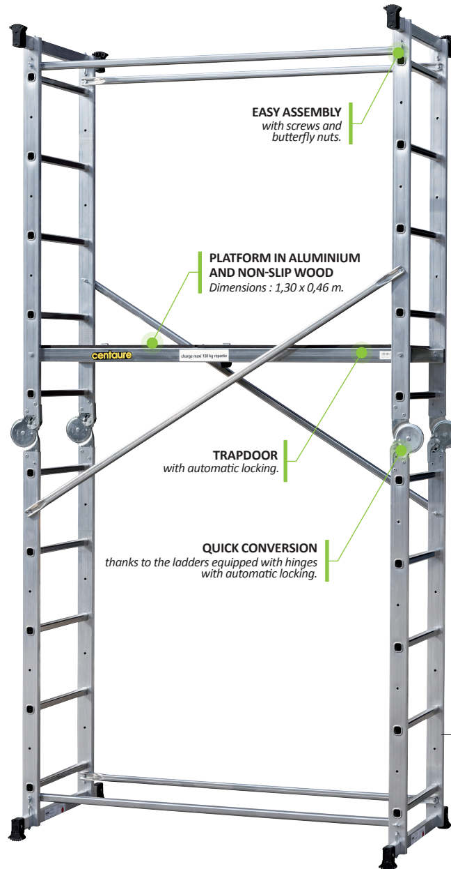
SCAFFOLD FOR OUTDOOR JOBS
